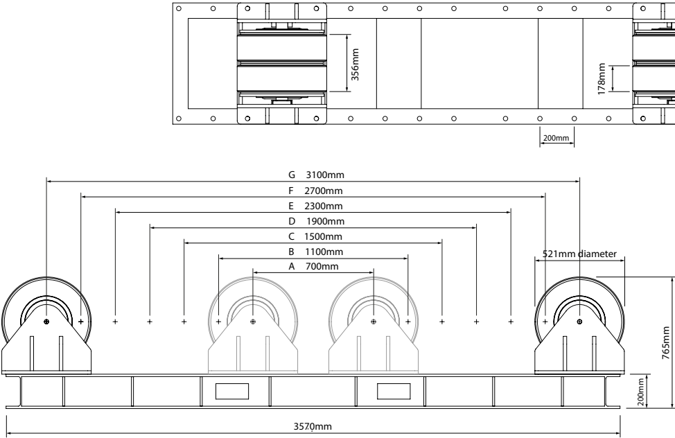
Wheel Setting Workpiece Diameter Range
